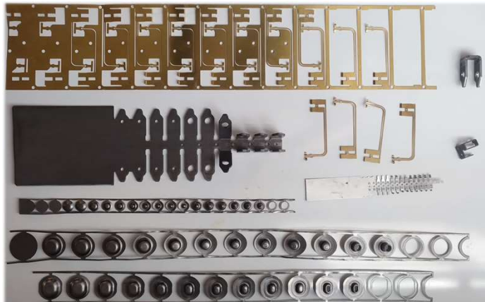
Alternator Parts
